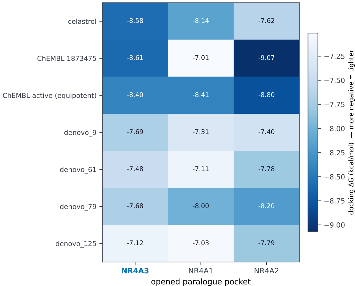
State-matched selectivity fingerprint (candidates × opened NR4A pockets; docking-tier priors)
