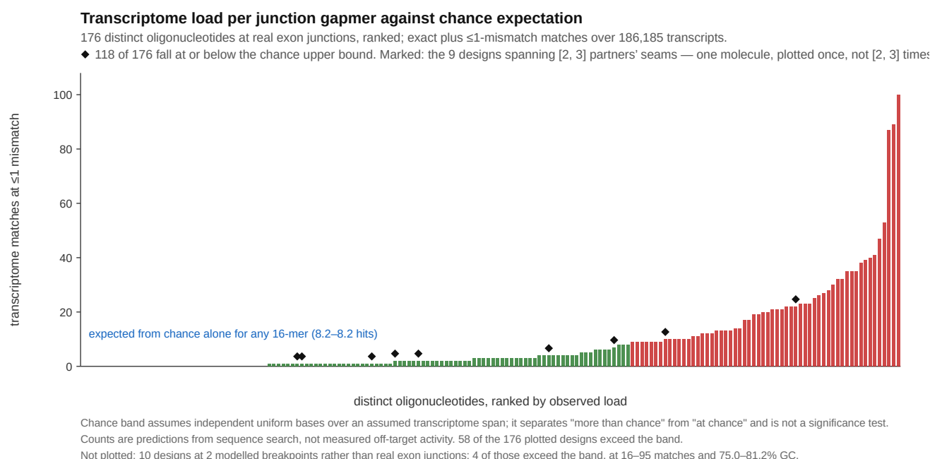
Figure 3. Transcriptome load per design against chance expectation. Each bar is one distinct oligonucleotide's count of exact plus \leq 1 -mismatch matches over 186,185 transcripts, ranked. The 190 design records at real exon junctions collapse to 176 molecules, because nine of the 16-mers are junction-spanning at more than one partner's junction at once — five at three junctions and four at two — and each of those is one physical oligonucleotide, plotted once rather than repeatedly (marked). The line is the number of such matches expected for an arbitrary 16-mer under an independent-uniform-base null, 8.2, computed against the scan's measured 718,571,139-nucleotide span; 118 of the 176 fall at or below it and 58 exceed it. Ten further designs from modelled breakpoints not built from a spliced transcript model are excluded, and are released with the artefacts. It is an expected count: the observed mean is 9.2, a ratio of 1.12, while the median is 3, so real transcript sequence produces a long right tail the null cannot rather than a uniform shift away from it. The line separates "more than chance" from "at chance" and is not a significance test; the counts are predictions from sequence search, not measured off-target activity.
