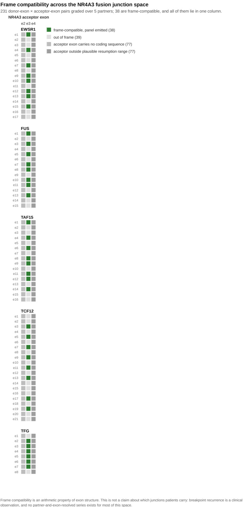
Figure 1. Reading-frame compatibility across the NR4A3 fusion junction space. All 231 donor-exon × acceptor-exon pairs across EWSR1 , TAF15 , TCF12 , FUS and TFG , graded against the frame condition. Rows are donor exons grouped by partner; columns are NR4A3 acceptor exons. Two acceptor columns are refused in every pair for structural reasons, so the 38 in-frame junctions lie in a single column.
