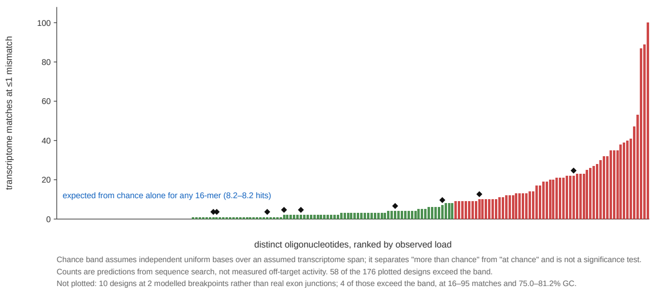
Figure 3. Transcriptome load per design against chance expectation. Each bar is one distinct oligonucleotide's count of exact plus \leq 1 -mismatch matches over 186,185 transcripts, ranked. The 190 design records at real exon junctions collapse to 176 molecules, because nine of the 16-mers are junction-spanning at more than one partner's junction at once — five at three junctions and four at two — and each of those is one physical oligonucleotide, plotted once rather than repeatedly (marked). The line is the number of such matches expected for an arbitrary 16-mer under an independent-uniform-base null, 8.2, computed against the scan's measured 718,571,139-nucleotide span; 118 of the 176 fall at or below it and 58 exceed it. Ten further designs from modelled breakpoints not built from a spliced transcript model are excluded, and are released with the artefacts. It is an expected count: the observed mean is 9.2, a ratio of 1.12, while the median is 3, so real transcript sequence produces a long right tail the null cannot rather than a uniform shift away from it. The line separates "more than chance" from "at chance" and is not a significance test; the counts are predictions from sequence search, not measured off-target activity.
