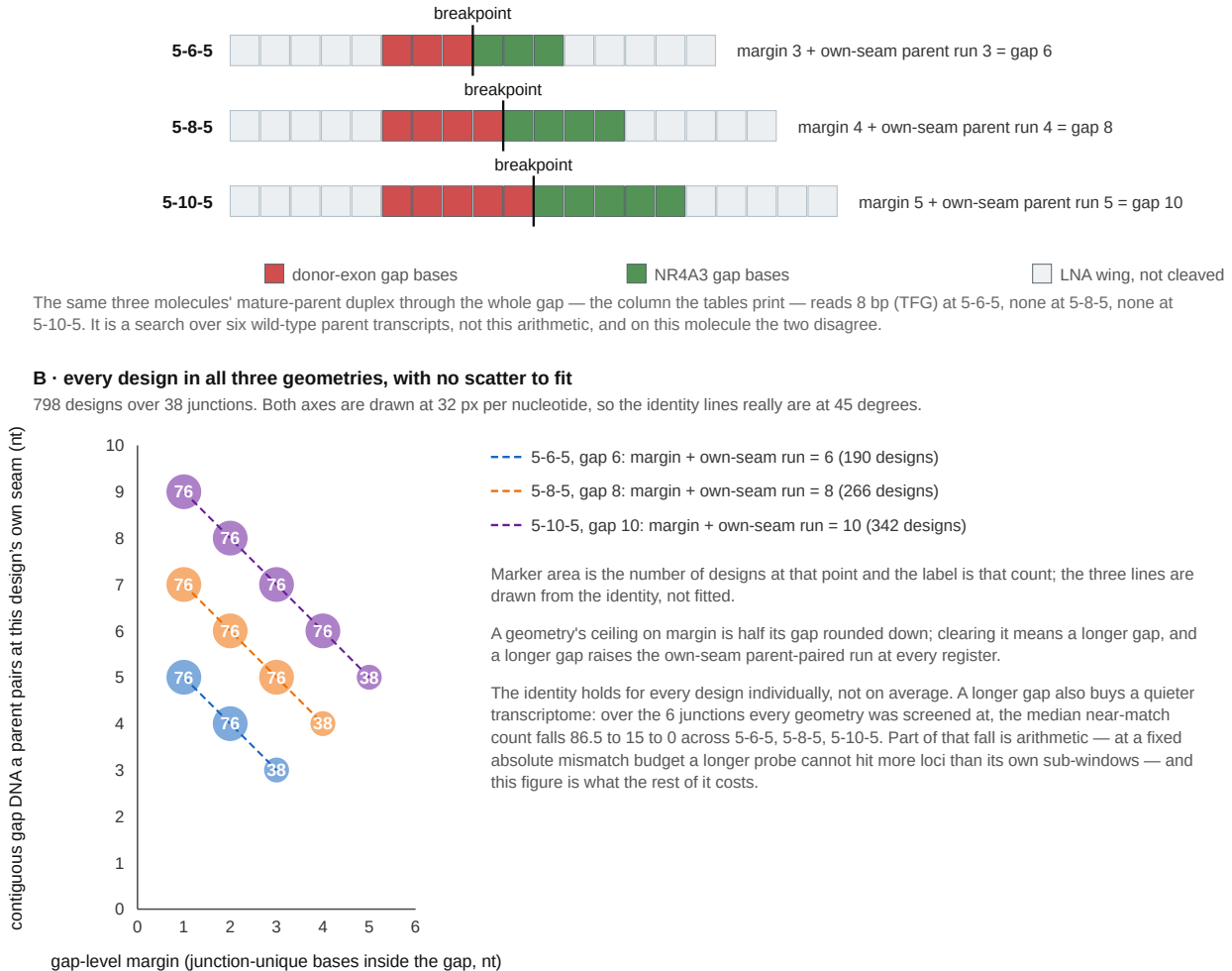
Figure 3. The margin a longer catalytic gap wins is the gap DNA a parent pairs at the design's own seam. (A) The best-margin design at EWSR1 exon 12 joined to NR4A3 exon 3, drawn at 5-6-5, 5-8-5 and 5-10-5 with the wings held at five nucleotides. Every base inside the catalytic gap comes from the donor exon or from the acceptor exon, so the junction-unique bases on the shorter side and the bases one wild-type parent pairs on the longer side tile the gap and sum to it. (B) Every fusion-specific design in all three geometries, 798 over 38 junctions, plotted as gap-level margin (abscissa) against the contiguous run of gap DNA one of the design's OWN two parents pairs at its seam (ordinate). That is not the quantity the markers and the do-not-order verdicts are set on. Those come from a SEARCH over all six mature parent transcripts, and the two separate: for the molecule drawn in (A) this figure draws 3 nucleotides where Tables 2, 3, 5 and 7 print an 8 bp duplex against wild-type TFG . The two also move in opposite directions across the geometries — the searched duplex FALLS (181 of 190, then 130 of 266, then 87 of 342 pair a parent at any length) and is flat at the ten-base-pair criterion (87, 88, 87), while the quantity drawn here RISES (76 of 190, 228 of 266, 342 of 342). A longer gap concedes seam-level parent DNA; it does not concede more of the liability this paper condemns. In (A) red marks the gap bases contributed by the donor exon, green those contributed by NR4A3 , and pale grey the LNA wings, which are not cleaved; the shorter of the two coloured runs is the margin and the longer is what a wild-type parent can pair, so which colour is which depends on the register — the junction drawn here divides its gap evenly in all three geometries, and 76 of the 190 designs at 5-6-5 have the longer run on the donor side; in (B) the three geometries are blue (5-6-5), orange (5-8-5) and purple (5-10-5). Both panels repeat these keys beside the drawing. Marker area is the number of designs at that point and the label is that count; the three lines are drawn from the identity, not fitted, and it holds for each
