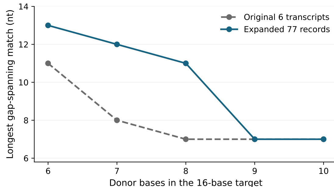
TCF12 junction: five binding positions
