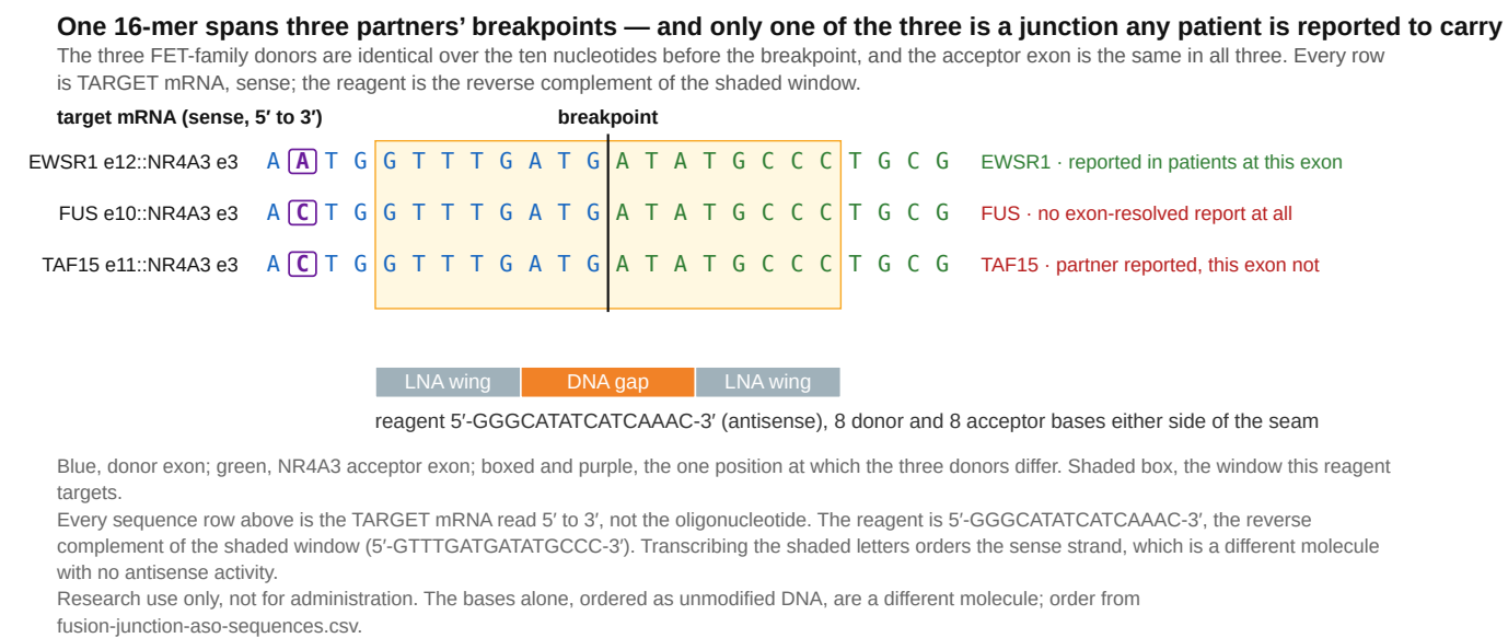
Figure 2. One 16-mer spans three partners' breakpoints. The junction windows of EWSR1 exon 12, TAF15 exon 11 and FUS exon 10 joined to NR4A3 exon 3, aligned at the breakpoint. Blue, donor exon; green, acceptor exon; positions at which the three donors differ are boxed as well as coloured, for greyscale and colour-blind readers. The shaded box is the target window of 5'-GGGCATATCATCAAAC-3', with the 5-6-5 locked-nucleic-acid (LNA)/DNA/LNA gapmer architecture below it; the note beneath the panel gives its gap-level margin of three. The three donors are the FET family — FUS , EWSR1 and TAF15 — and they are identical over the ten nucleotides before the breakpoint, which is what makes one oligonucleotide junction-spanning at all three junctions. Two of the three drawn junctions are not reported in any patient: the exon-resolved TAF15 breakpoints in this disease are at exon 6 rather than exon 11, and no exon-resolved FUS breakpoint has been published at all (§2.2). This is a statement about sequence, not a claim that one reagent serves three patient groups. Coverage is predicted from sequence and has not been measured.
