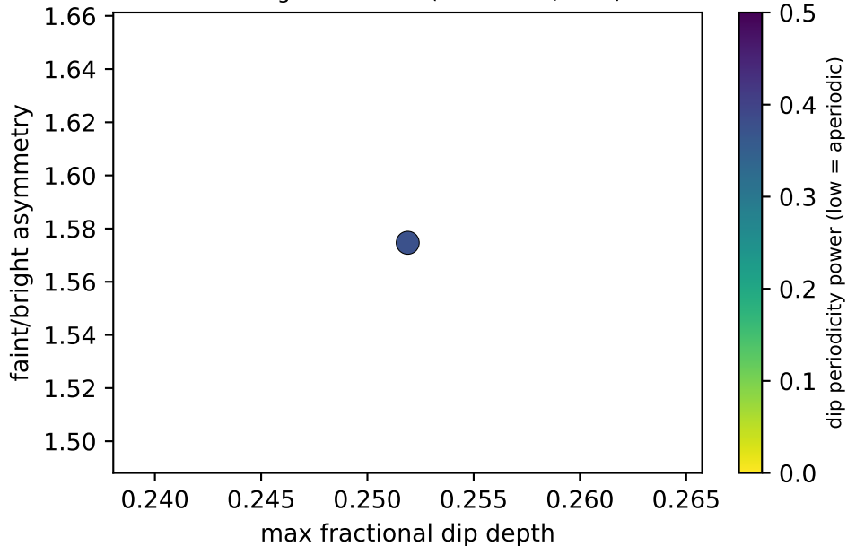
Dimming candidates (field 175.0, 28.0)
