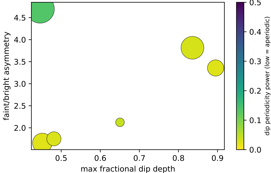
Dimming candidates (field 190.0, 30.0)
