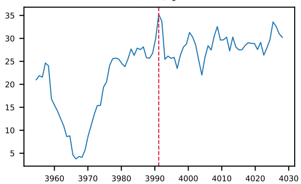
0577e38d \lambda=3991.2 S/N=8, rg*
