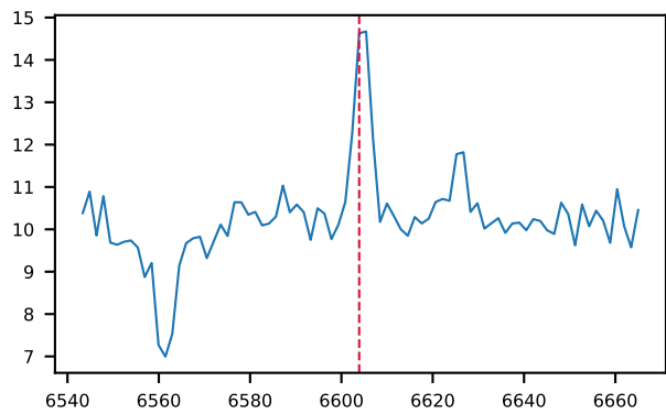
00ac8d30 \lambda=6602.4 S/N=24, ag?
