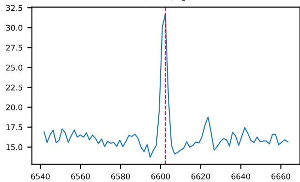
00ac8d30 \lambda=6602.4 S/N=24, ag?
