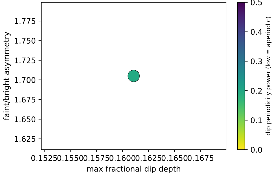
Dimming candidates (field 128.0, 22.0)
