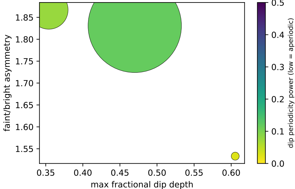
Dimming candidates (field 270.0, 30.0)
