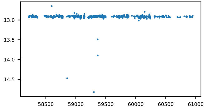
630209400000 depth=0.54, n_dip=12, asym=1.5
