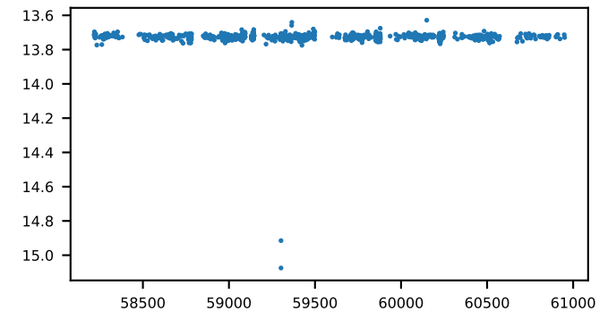
167520320002 depth=0.13, n_dip=3, asym=1.5
