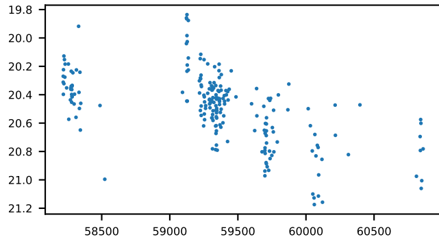
630209400000 depth=0.54, n_dip=12, asym=1.5
