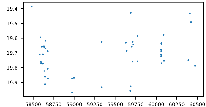
167520320000 depth=0.27, n_dip=5, asym=1.5
