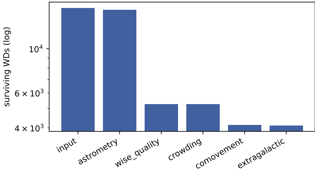
Empirical contamination funnel (100 pc)
