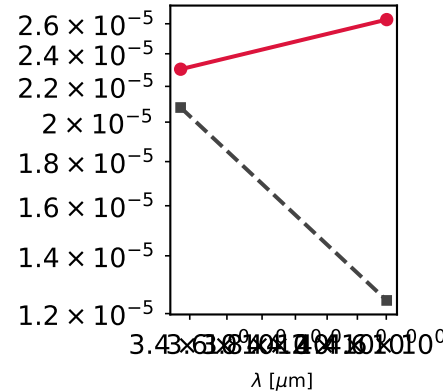
WD 6141704453328101632 Teff=5440K
