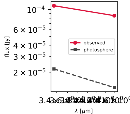
WD 1289022219283937408 Teff=4285K
