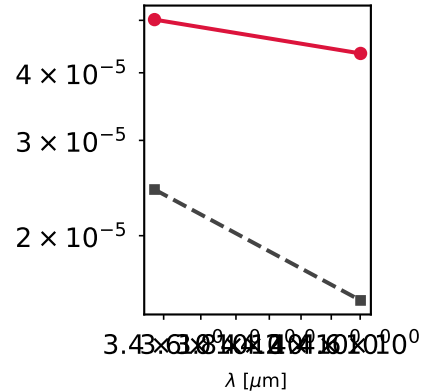
WD 2984105588925961728 Teff=4130K
