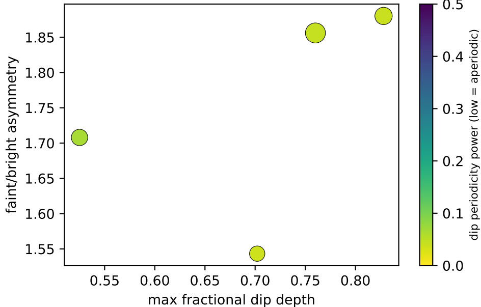
Dimming candidates (field 165.0, 50.0)
