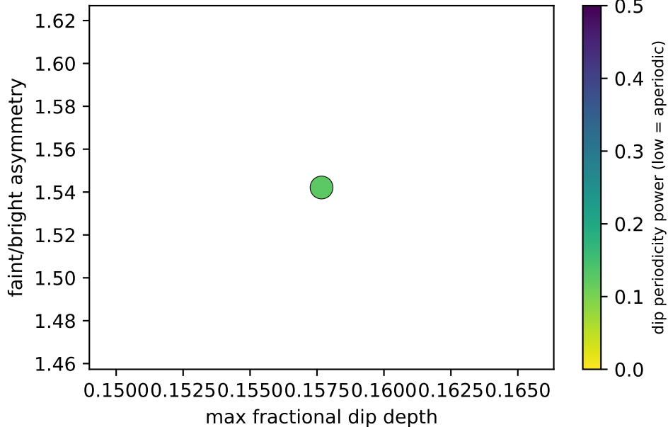
Dimming candidates (field 155.0, 18.0)
