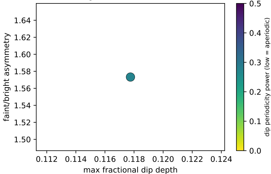
Dimming candidates (field 130.0, 35.0)
