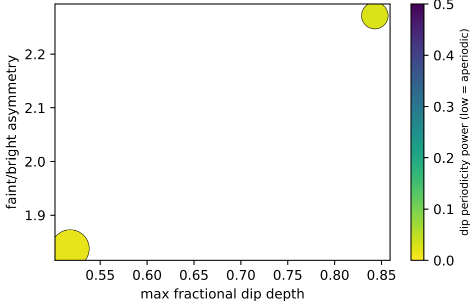
Dimming candidates (field 210.0, 45.0)
