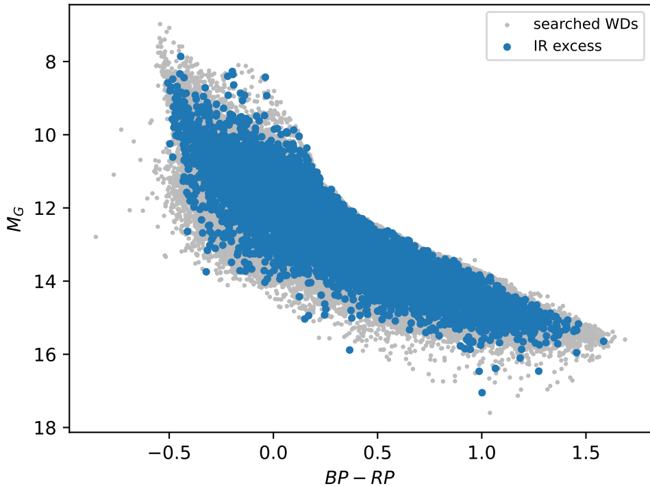
White-dwarf sample (Gaia HR diagram)
