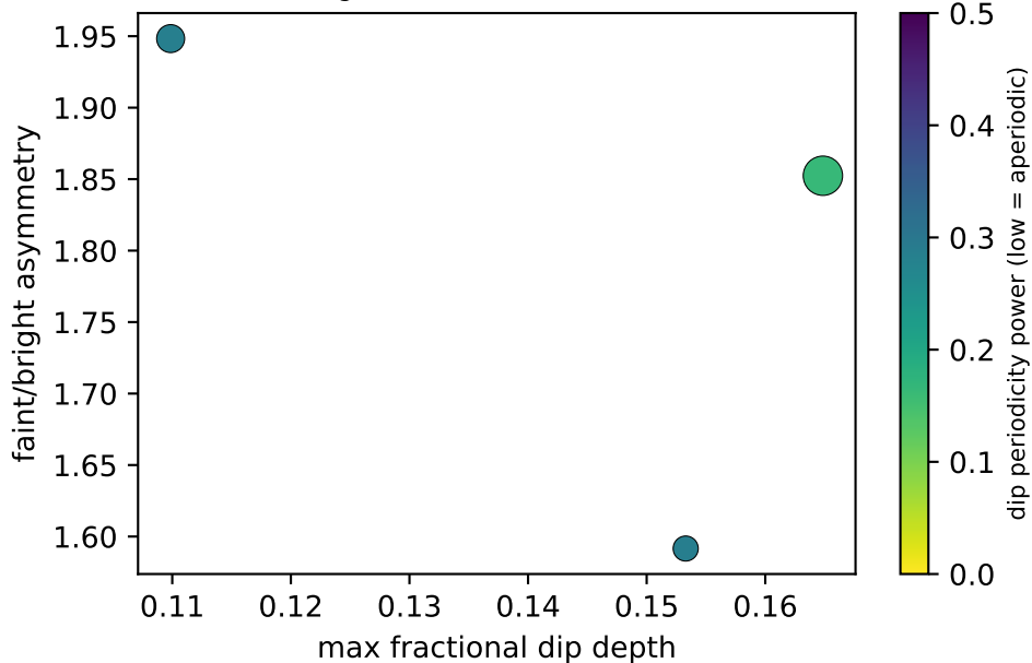
Dimming candidates (field 130.0, 25.0)
