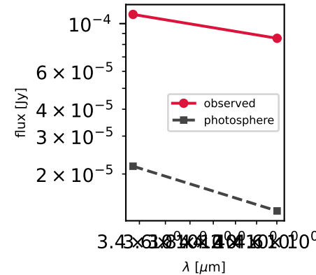
WD 1289022219283937408 Teff=4285K
