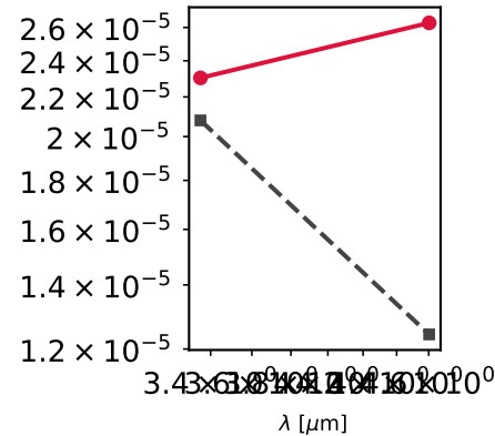
WD 6141704453328101632 Teff=5440K
