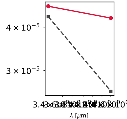
WD 1091005054206114304 Teff=4760K
