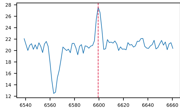
04c8c3be \lambda=4753.4 S/N=8, unexamined
