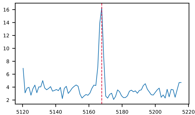
06555124 \lambda=6853.3 S/N=14, unexamined
