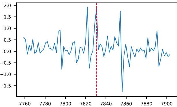
06074d57 \lambda=7830.7 S/N=8, unexamined
