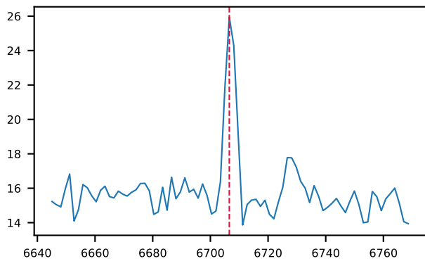
04854012 \lambda=6706.6 S/N=20, unexamined
