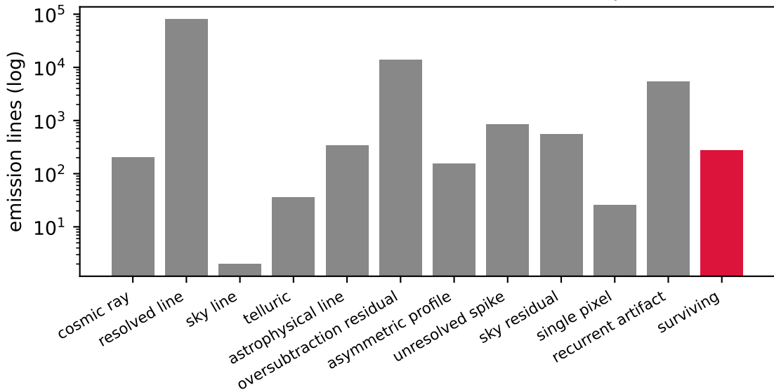
Laser-line funnel: SDSS-DR17, 22,500 spectra
