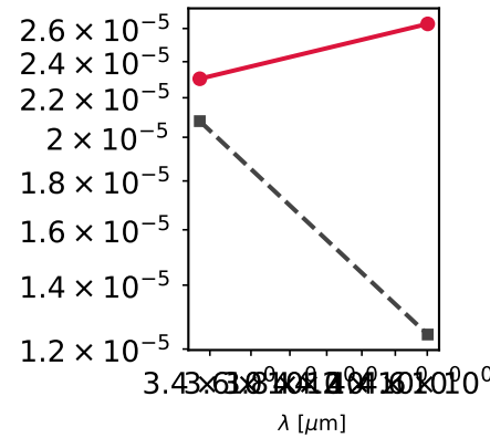
WD 6141704453328101632 Teff=5440K
