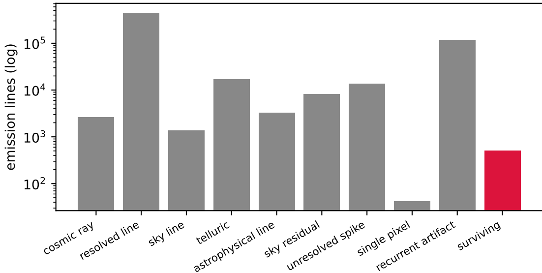
Laser-line funnel: DESI-DR1, 60,000 spectra
