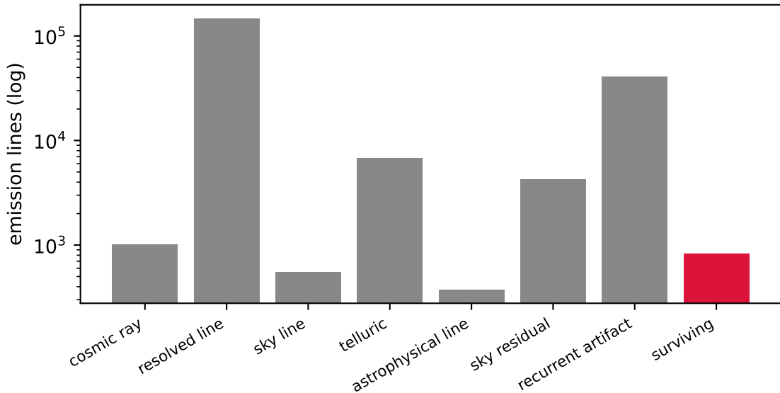
Laser-line funnel: DESI-DR1, 20,000 spectra
