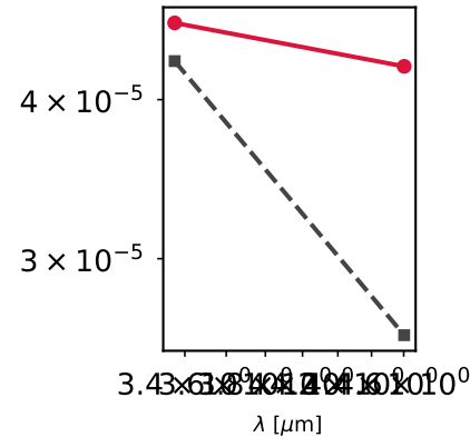
WD 1091005054206114304 Teff=4760K
