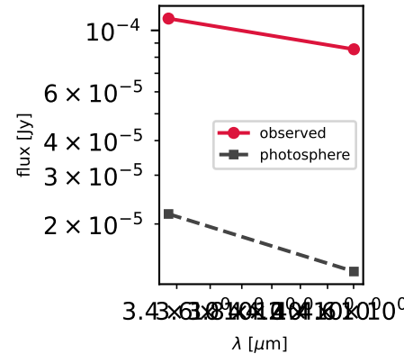
WD 1289022219283937408 Teff=4285K
