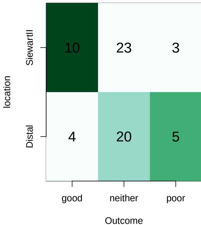
Outcome Chisq = 0.28
