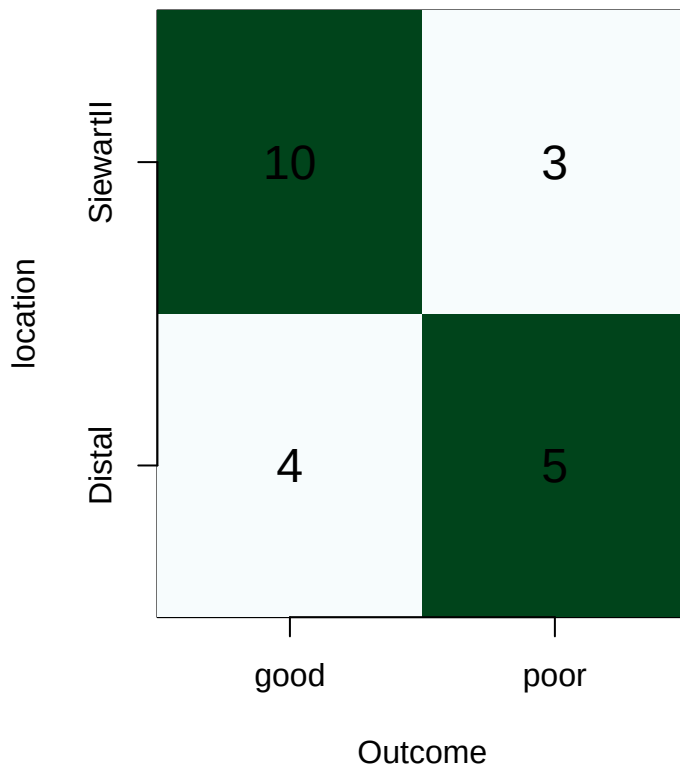
Outcome Chisq = 0.27
