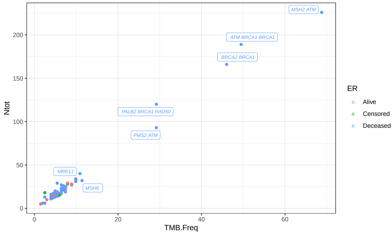
Tumour coding burden vs total mutations
