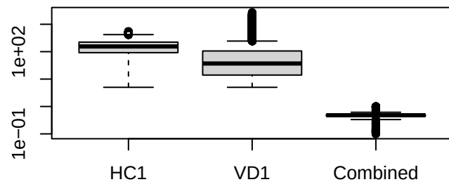
nALT
