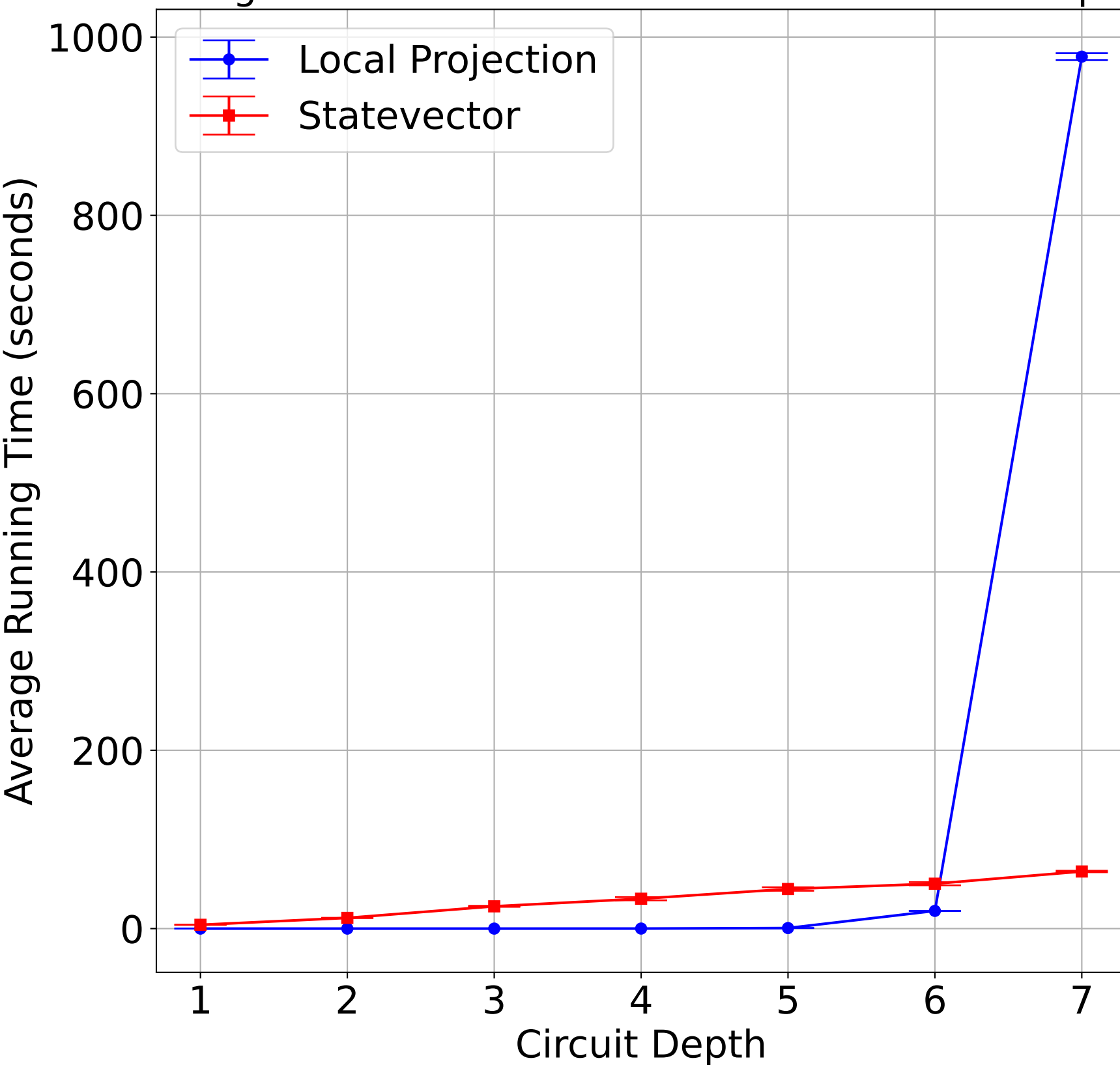
Running Time for 100 Haar Random Circuits of 30 qubits
