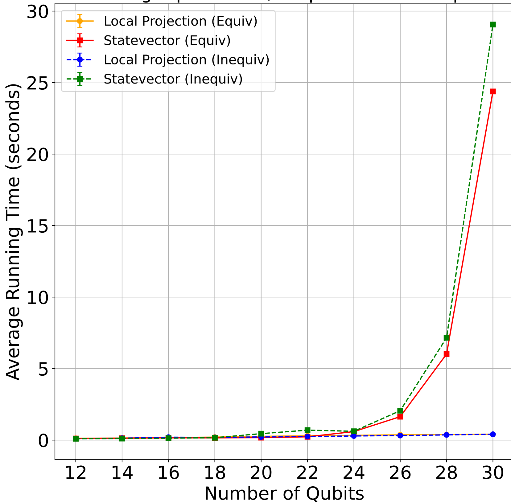
Checking Equivalence/Inequivalence at depth 3
