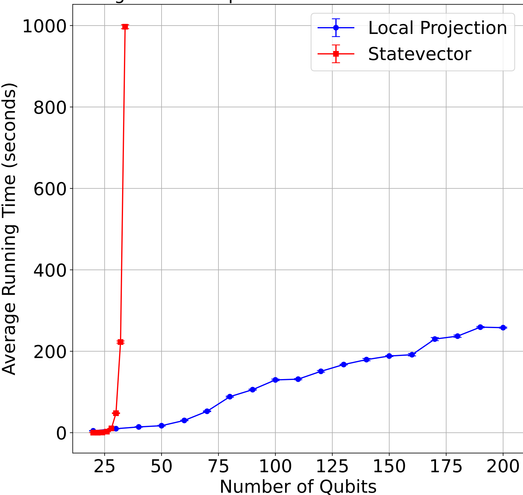
Running Time at Depth 6 for 100 Haar Random Circuits
