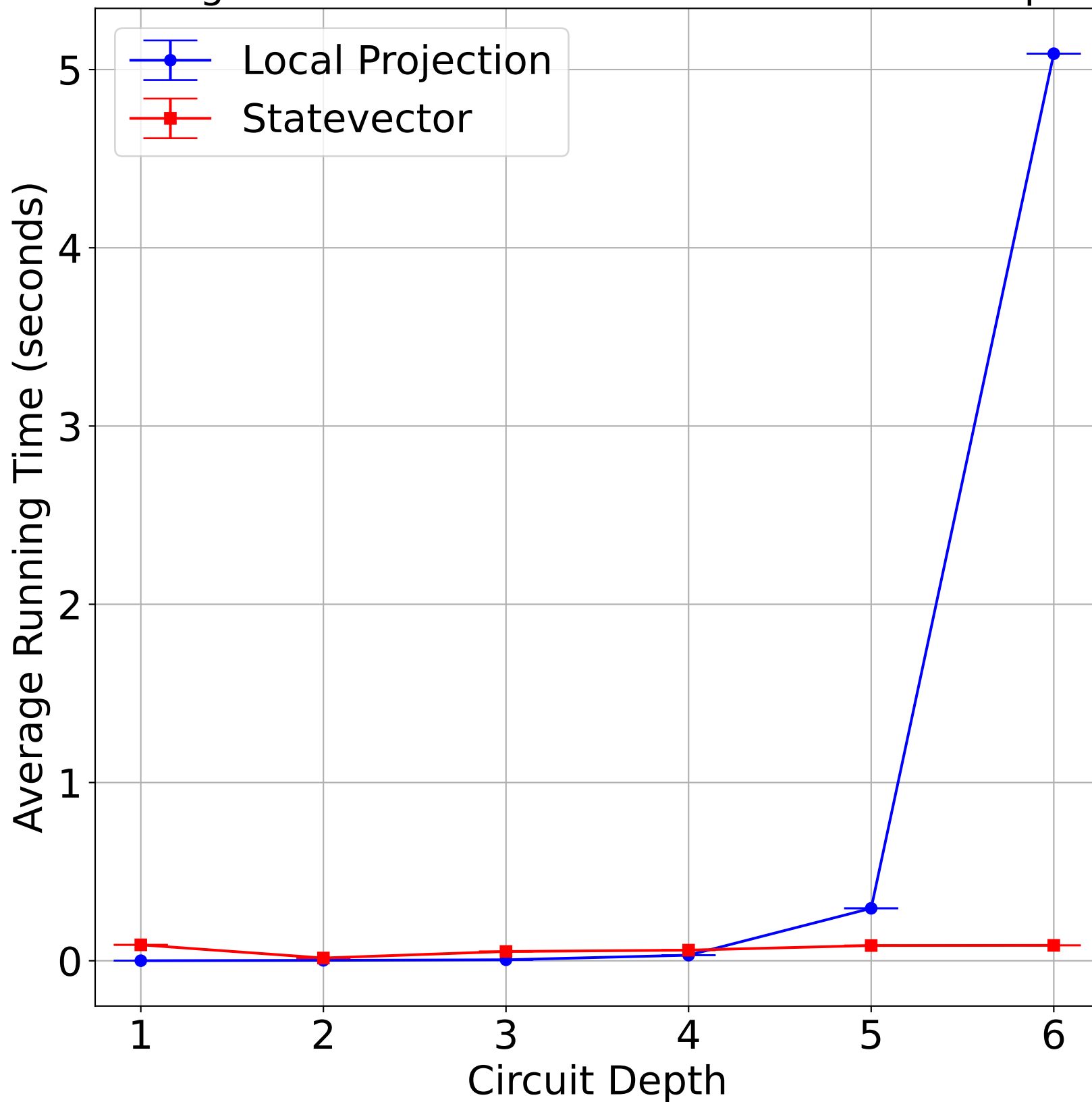
Running Time for 1 Haar Random Circuits of 20 qubits
