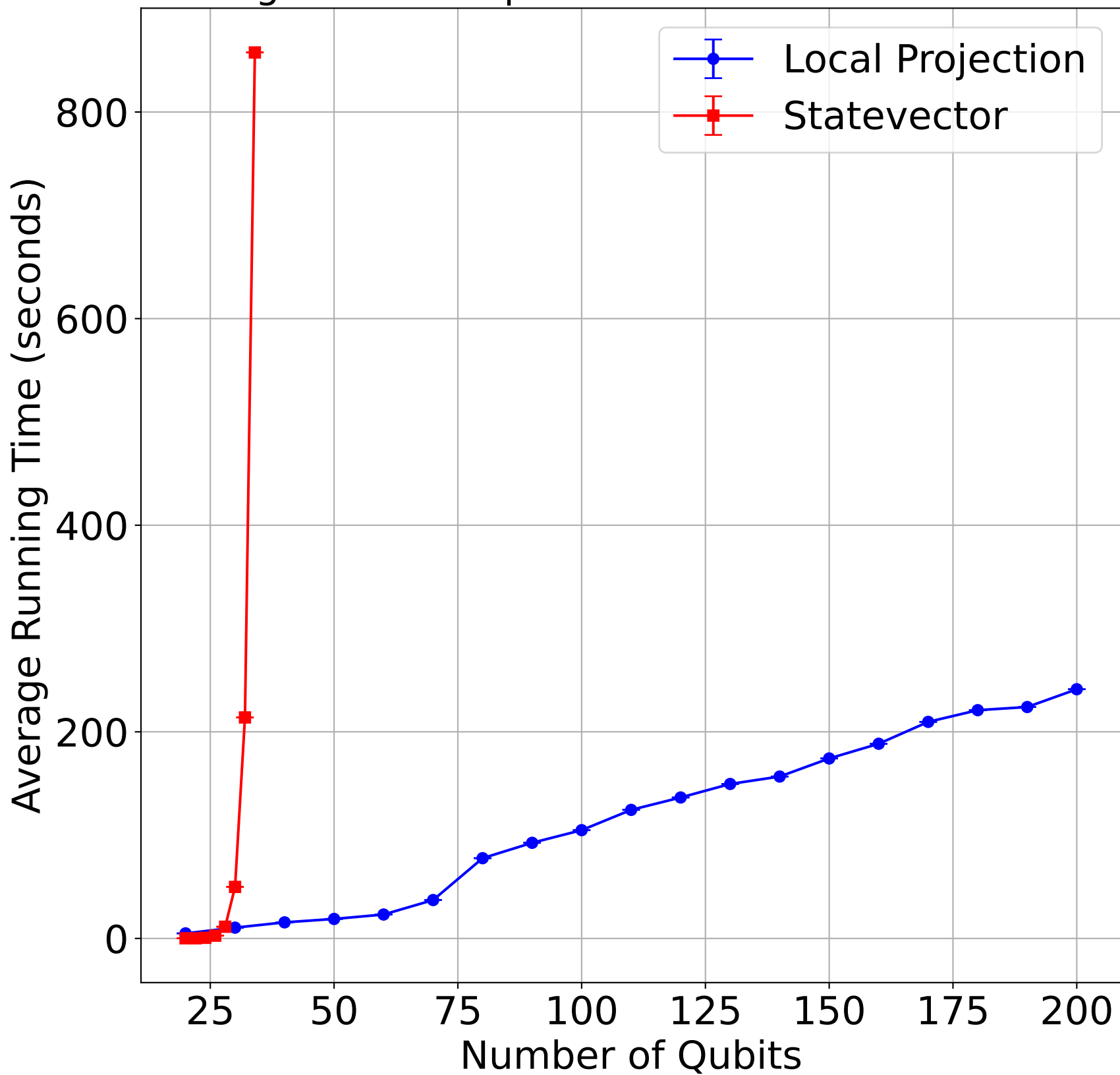
Running Time at Depth 6 for 1 Haar Random Circuits
