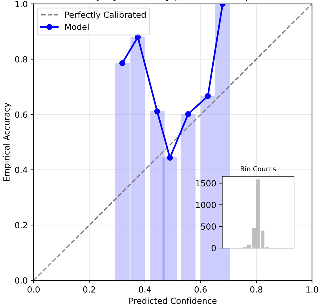
Reliability Diagram: SimpleKT (Very Sparse KCs) Dataset: Junyi Academy | ECE: 0.0841 | N: 2,545
