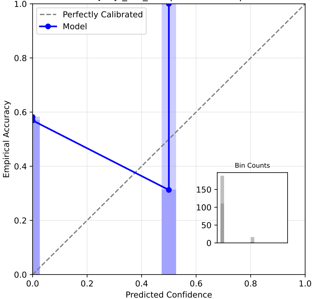
Reliability Diagram: bkt (very_sparse) Dataset: junyi_bkt_test | ECE: 0.5317 | N: 1264
