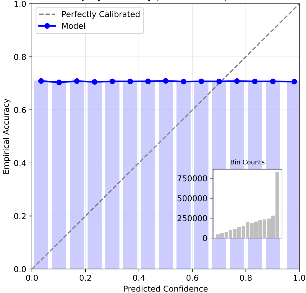
Reliability Diagram: SimpleKT (Dense KCs) Dataset: Junyi Academy | ECE: 0.2267 | N: 3,072,767
