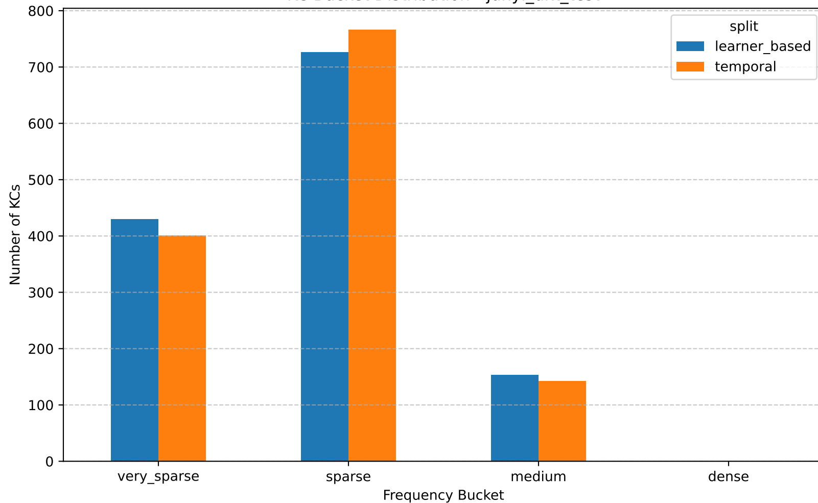
KC Bucket Distribution - junyi_dkt_test
