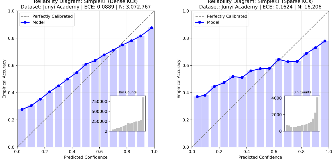
(a) Reliability diagram of SimpleKT on Junyi temporal split for Dense KCs.
