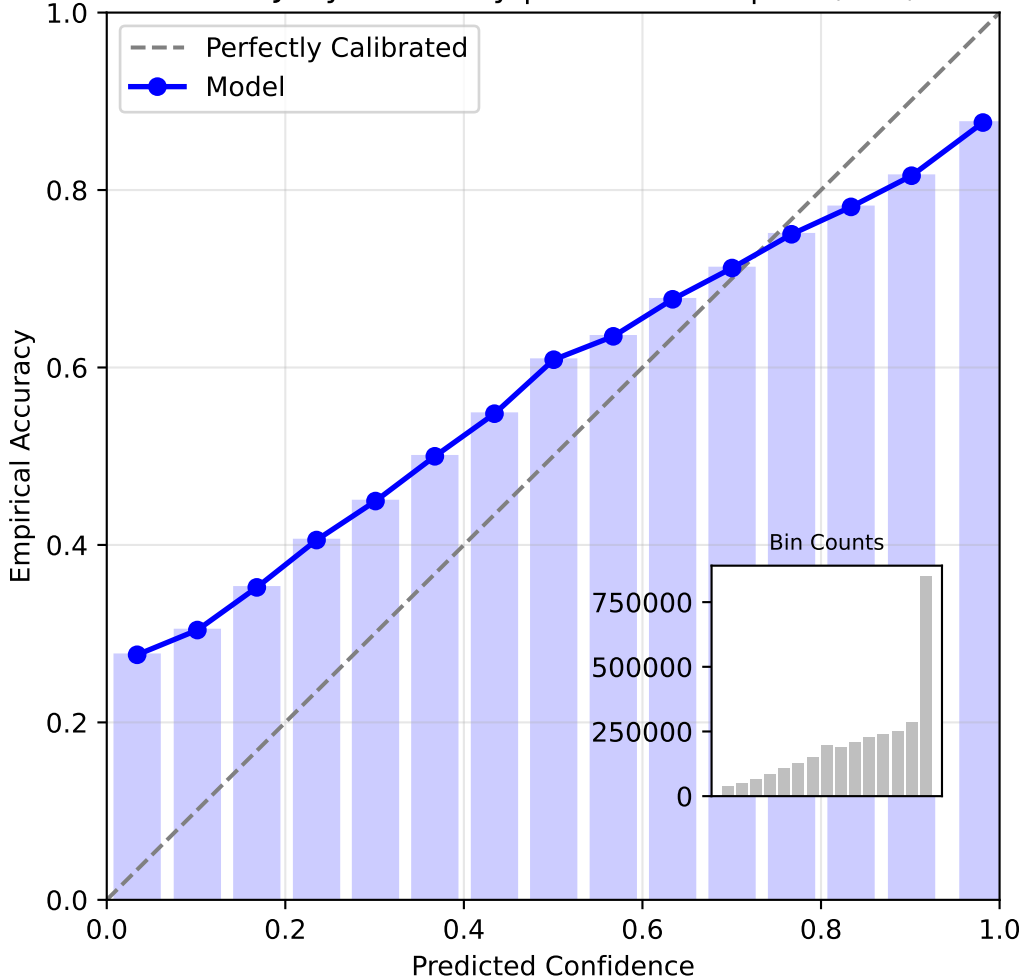
Reliability Diagram: SimpleKT (Dense KCs) Dataset: Junyi Academy | ECE: 0.0889 | N: 3,072,767
