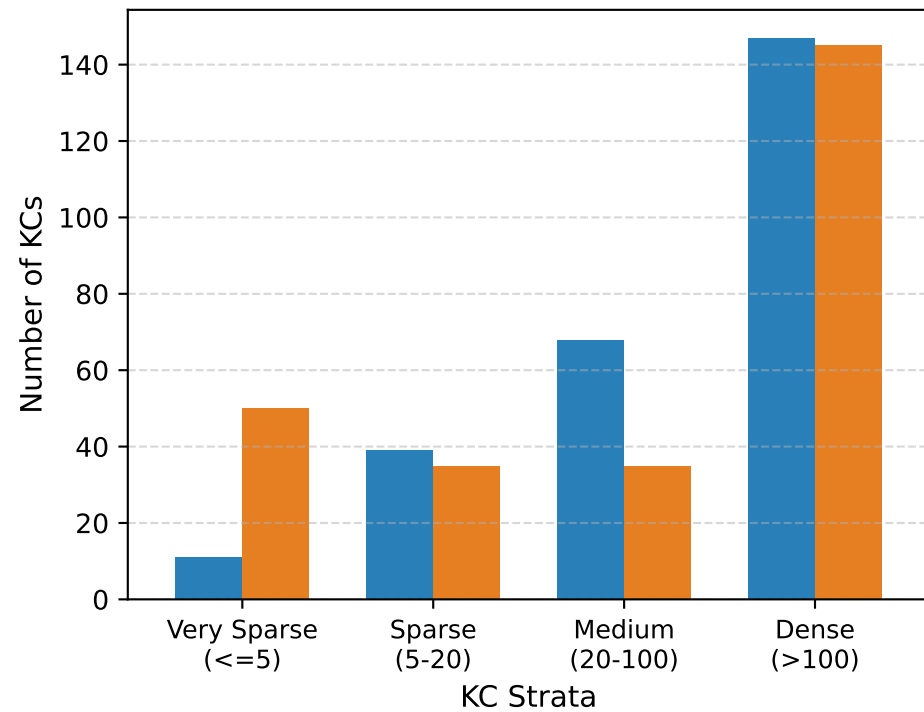
ASSISTments 2012
