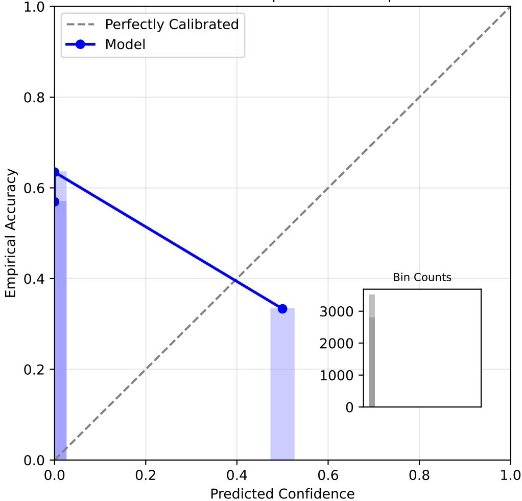
Reliability Diagram: bkt (medium) Dataset: assist2012 | ECE: 0.5693 | N: 5677
