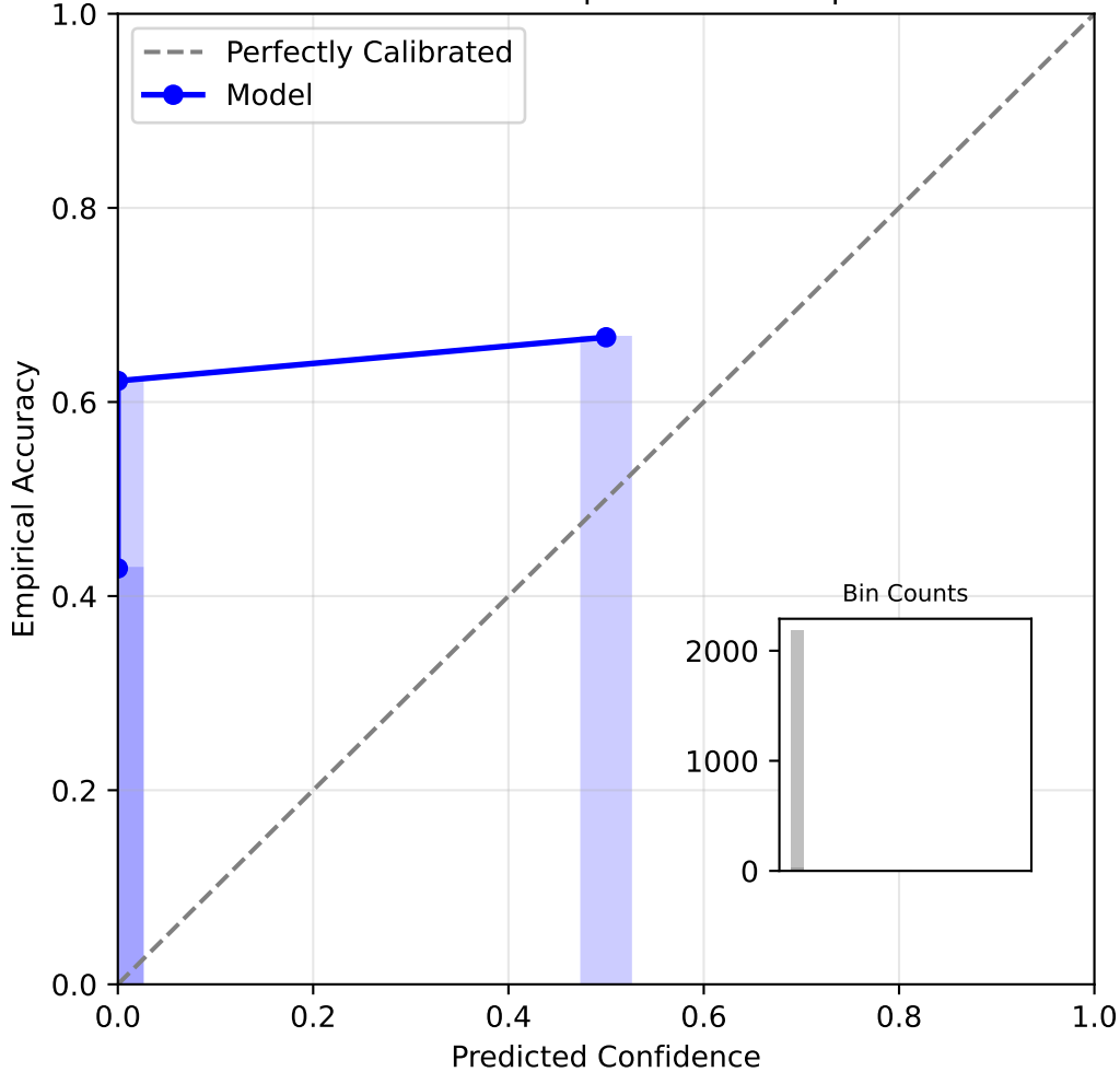
Reliability Diagram: bkt (sparse) Dataset: assist2012 | ECE: 0.6211 | N: 3030
