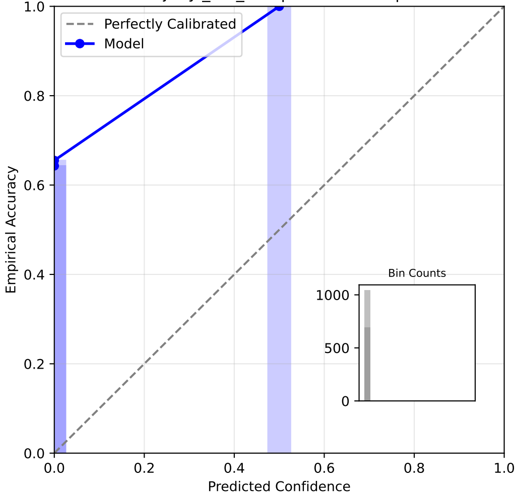
Reliability Diagram: bkt (medium) Dataset: junyi_bkt_test | ECE: 0.6546 | N: 5780
