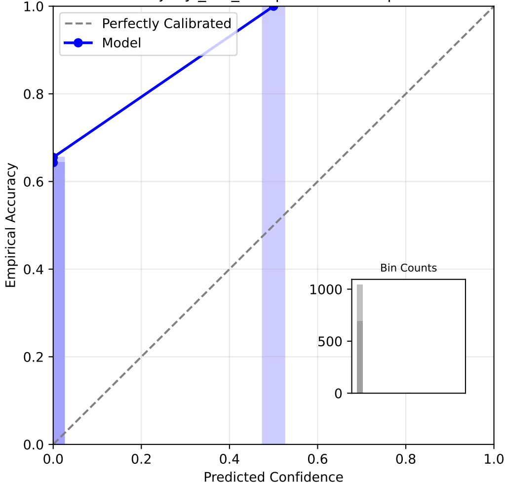
Reliability Diagram: bkt (medium) Dataset: junyi_bkt_test | ECE: 0.6430 | N: 6597
