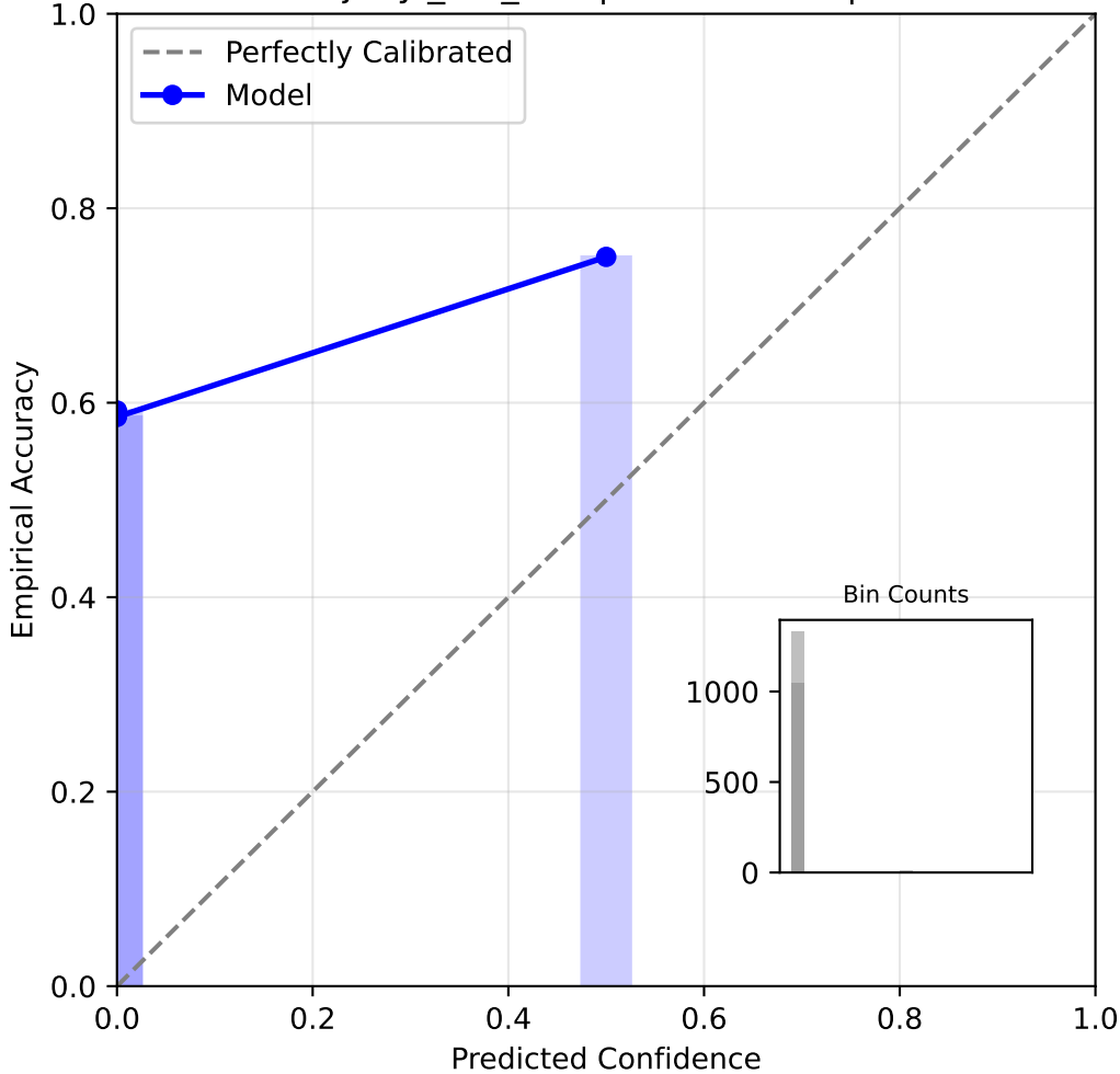
Reliability Diagram: bkt (sparse) Dataset: junyi_bkt_test | ECE: 0.5834 | N: 10589
