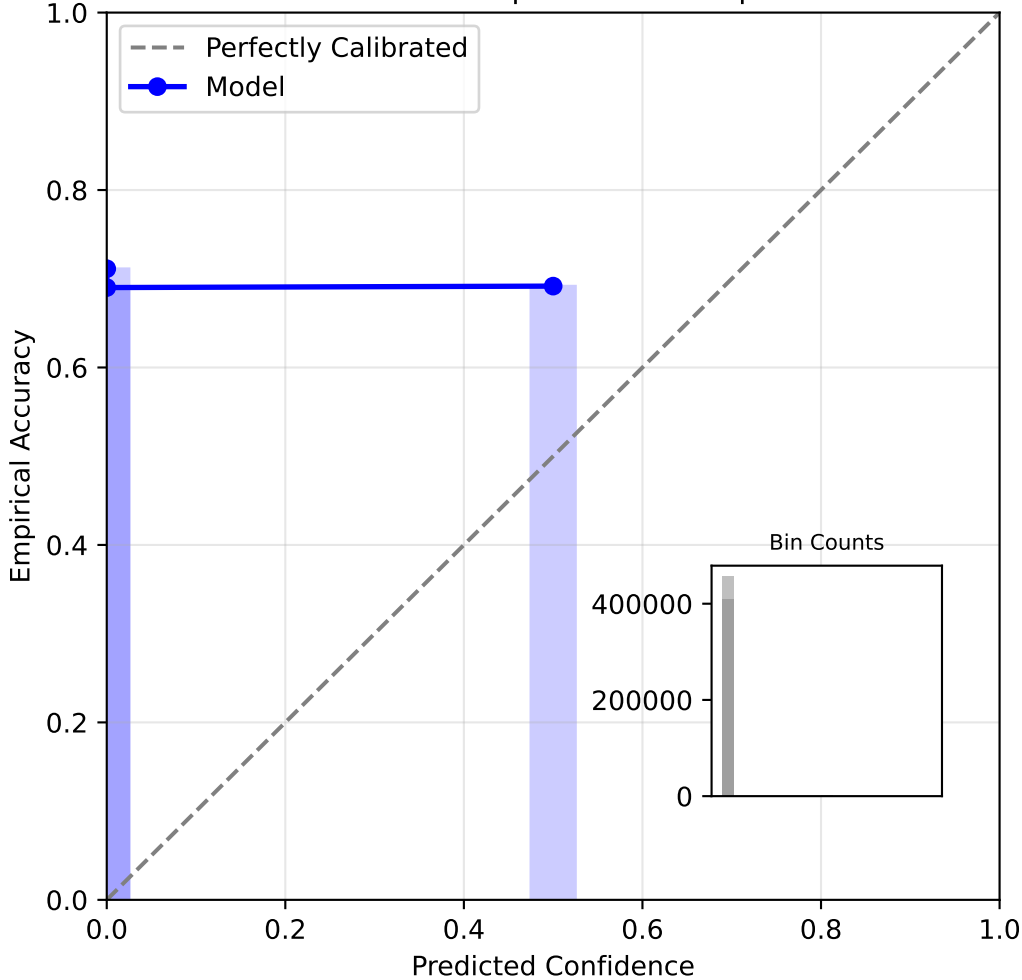
Reliability Diagram: bkt (dense) Dataset: assist2012 | ECE: 0.6884 | N: 521661
