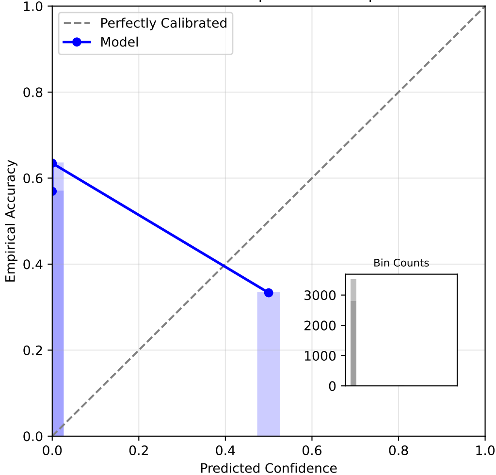
Reliability Diagram: bkt (medium) Dataset: assist2012 | ECE: 0.6340 | N: 4558
