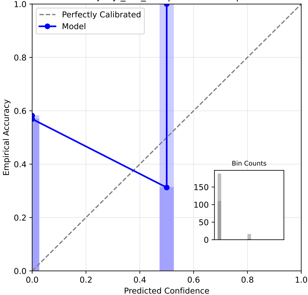
Reliability Diagram: bkt (very_sparse) Dataset: junyi_bkt_test | ECE: 0.5684 | N: 1391
