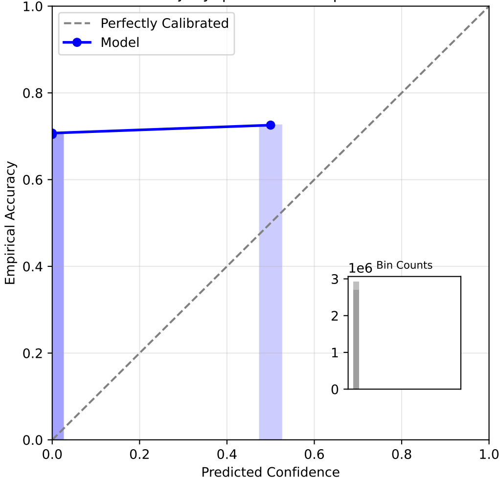
Reliability Diagram: bkt (dense) Dataset: junyi | ECE: 0.7041 | N: 3264405
