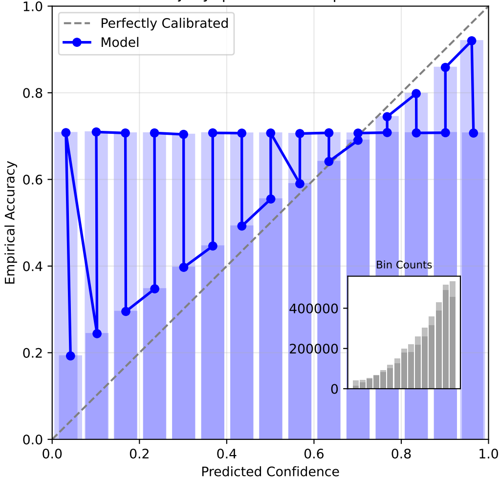
Reliability Diagram: dkt (dense) Dataset: junyi | ECE: 0.0405 | N: 3264405
