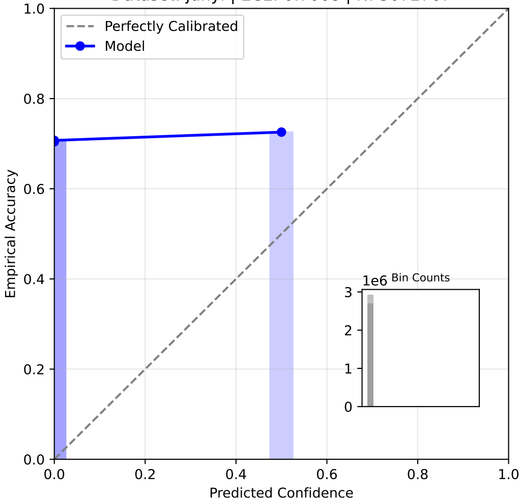
Reliability Diagram: bkt (dense) Dataset: junyi | ECE: 0.7068 | N: 3072767
