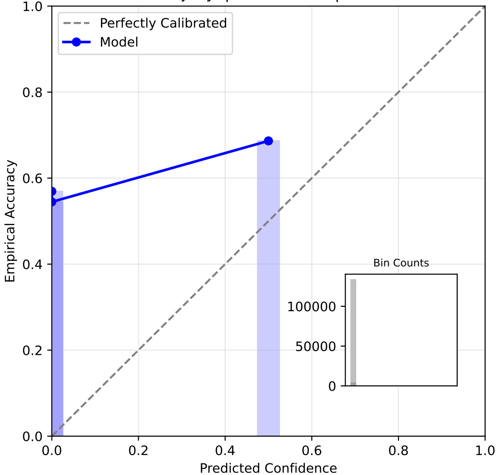
Reliability Diagram: bkt (medium) Dataset: junyi | ECE: 0.5446 | N: 151597
